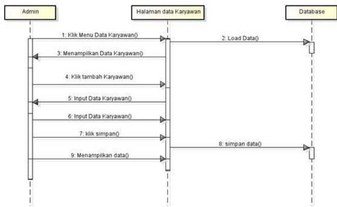
Gambar 4 Sequence Diagram Create Karyawan
