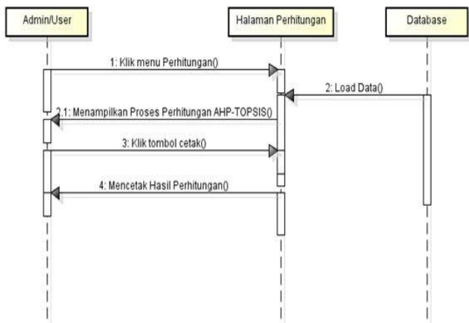
Gambar 5 Sequence Diagram Hasil Perhitungan AHP-TOPSIS
