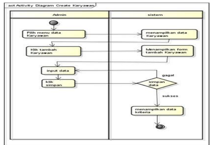
Gambar 2 Activity Diagram Create Karyawan
