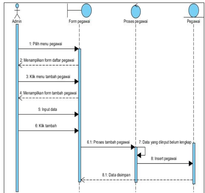
Gambar 4. Sequence Diagram Tambah Pegawai
