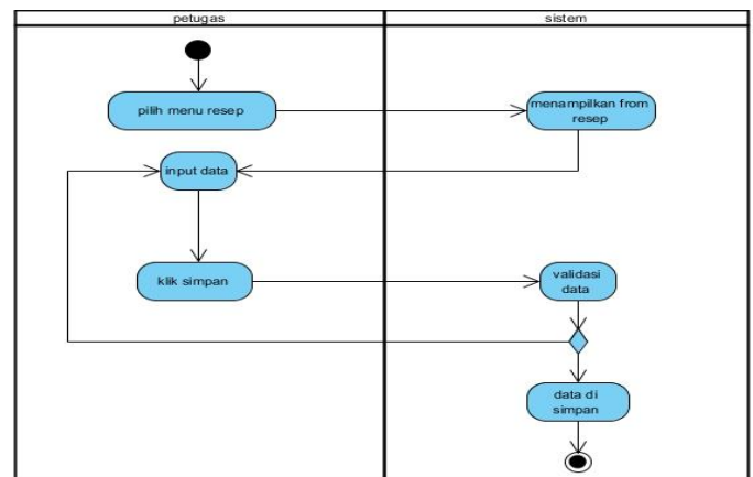
Gambar 9. Activity Diagram Resep
