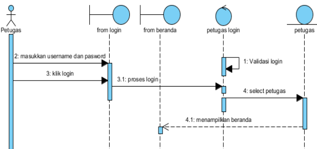
Gambar 16. Sequence Diagram Login
