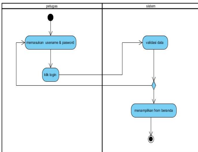
Gambar 7. Activity Diagram Menu Login
