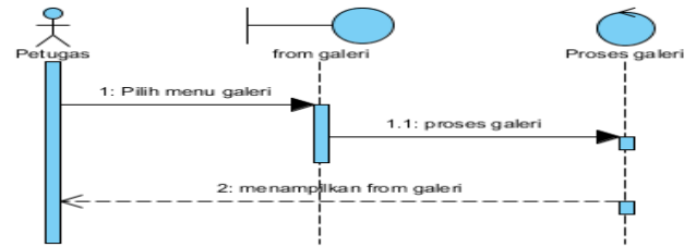
Gambar 17. Sequence Diagram Galeri
