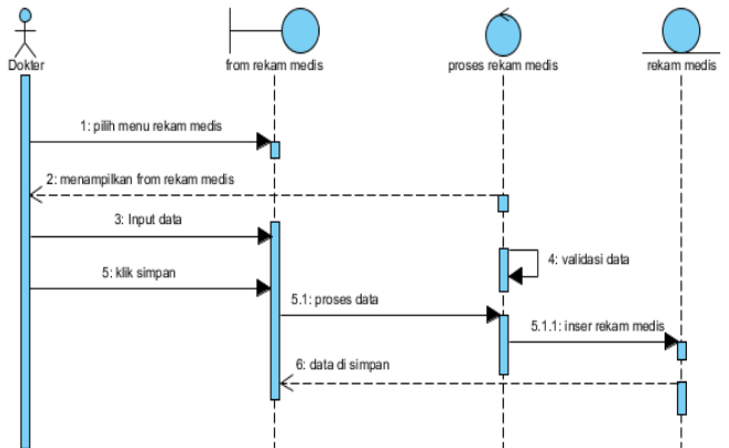
Gambar 17. Sequence Diagram Rekam Medis
