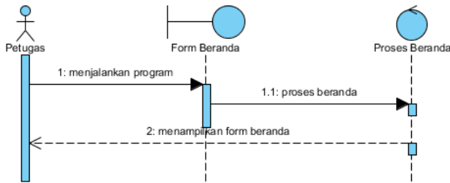
Gambar 15. Sequence Diagram Beranda
