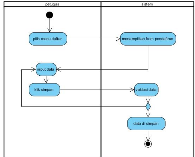
Gambar 8. Activity Diagram Pendaftaran
